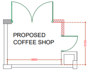
COFFEE SHOP PLAN
