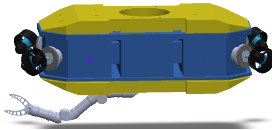
Fig. 1. Conceptual design of the proposed vehicle manipulator system
