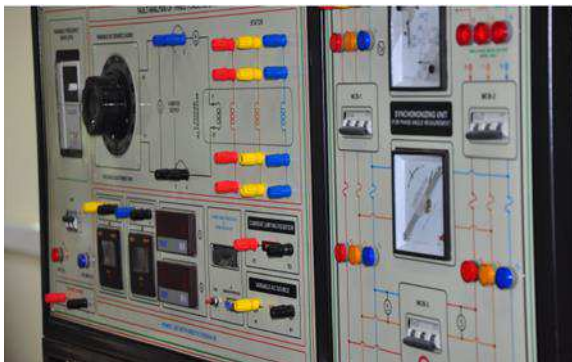
Power Systems Lab, Left: Alternator Fault Simulator wWith Grid Synchronization Facility, Right: Solar Photo Voltaic Array Simulator
